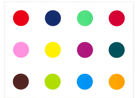
Methionine
