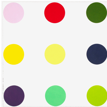
Phenformin
