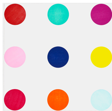
Tryptophan
