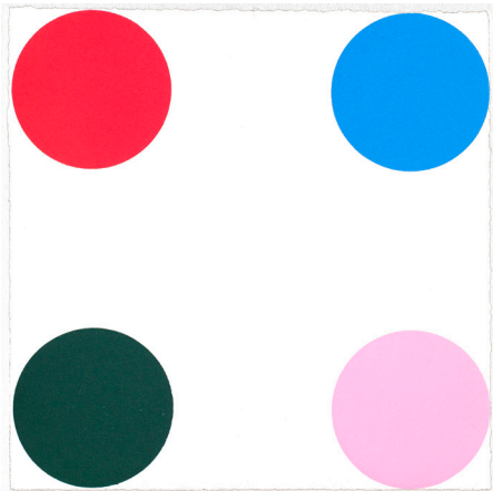
Cyclizine
