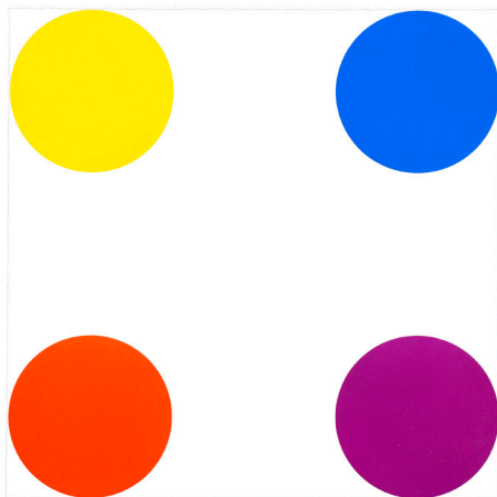
Norleucine
