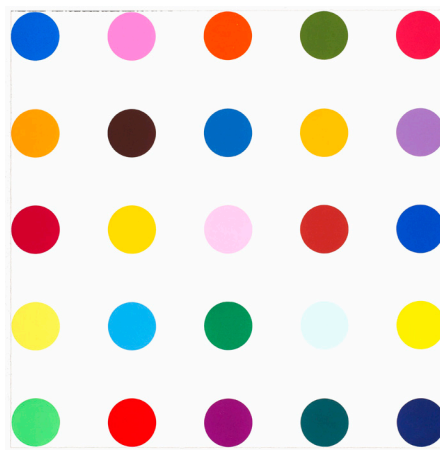
Bromobenzotrifluoride
