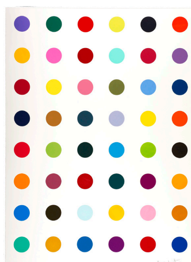
Hydroxylysine
