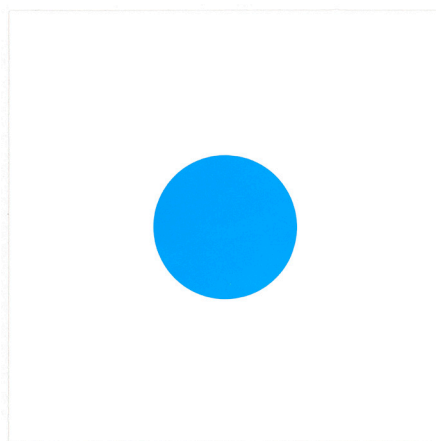
Pridinol
