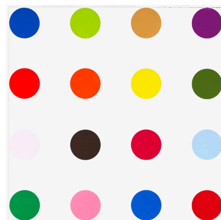
Coccarboxylase
